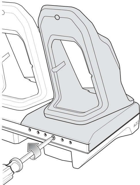
Figure 2-35 Remove Screw
